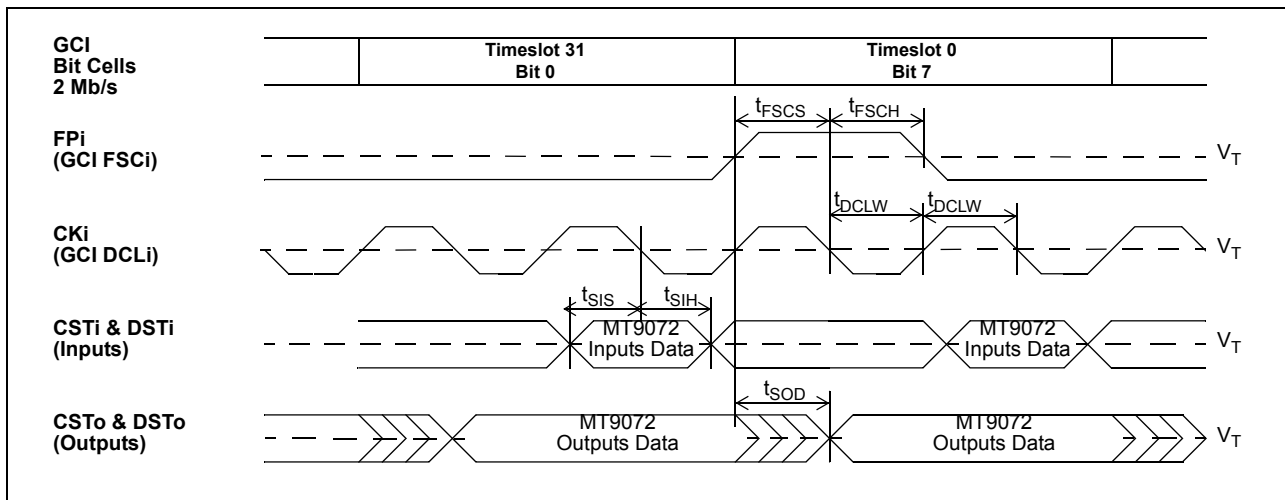
Figure 32 - GCI 2.048 Mb/s Timing Diagram
