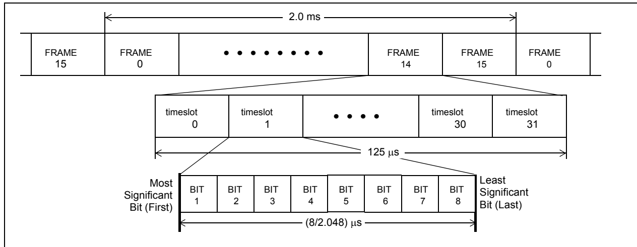
Figure 55 - PCM 24 Format
