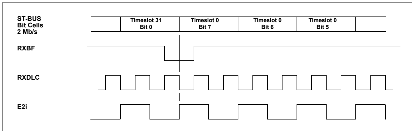
Figure 58 - Receive IMA Functional Timing Diagram
