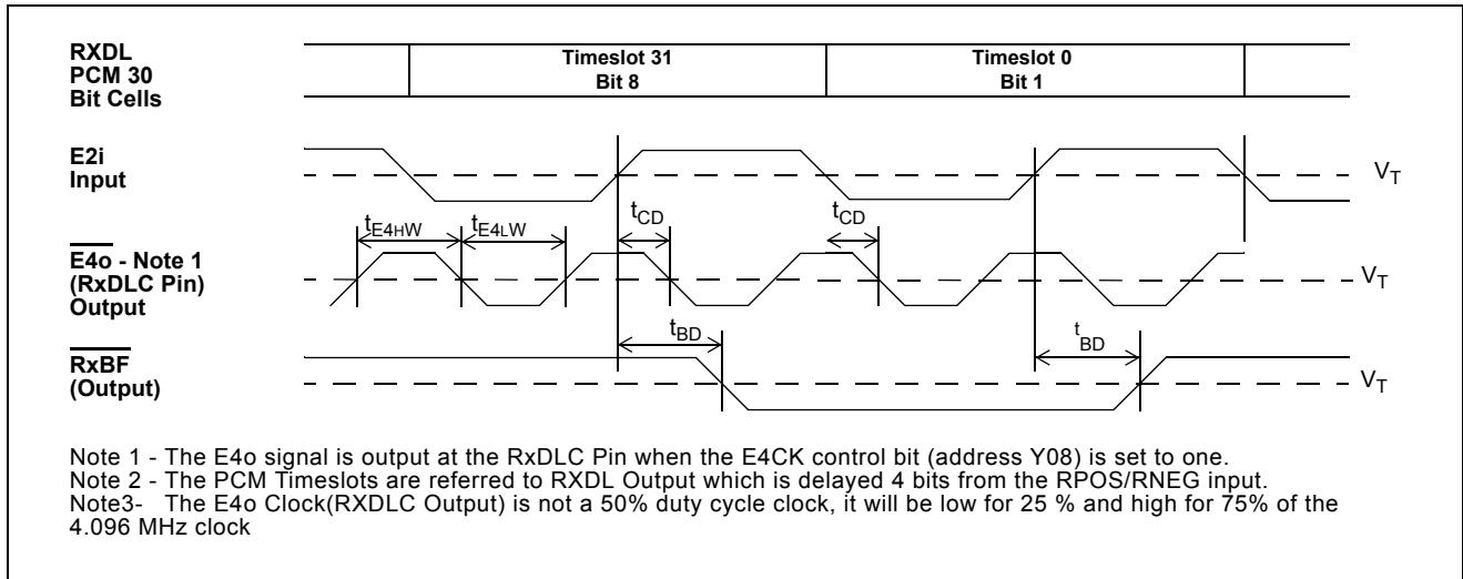
Figure 67 - Receive Basic Frame and \overline{\text{E4o}} Timing
