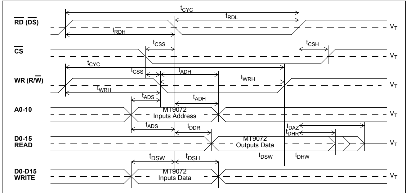
Figure 29 - Intel Microprocessor Timing
