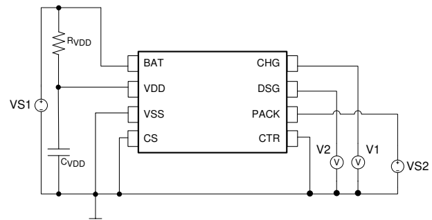
Figure 9-2. Test Circuit 2
