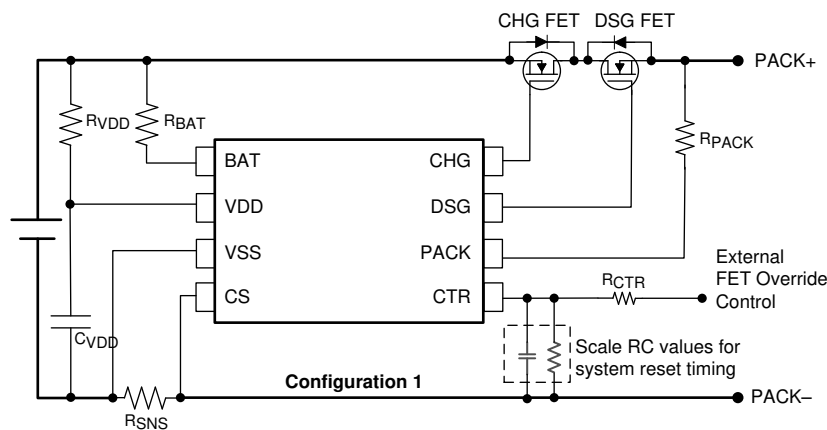
Figure 9-6. BQ298x Reference Schematic Configuration 1
