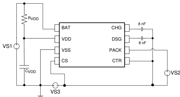
Figure 9-3. Test Circuit 3
