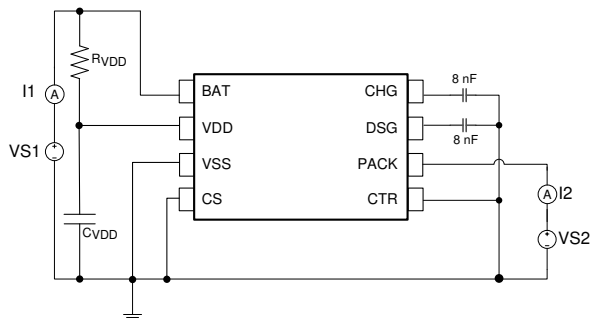
Figure 9-1. Test Circuit 1
