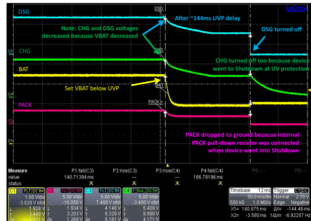
Figure 9-9. Undervoltage (UV) Protection
