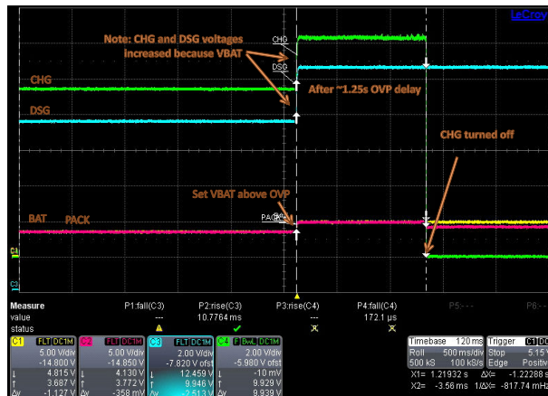
Figure 9-8. Overtolerance (OV) Protection
