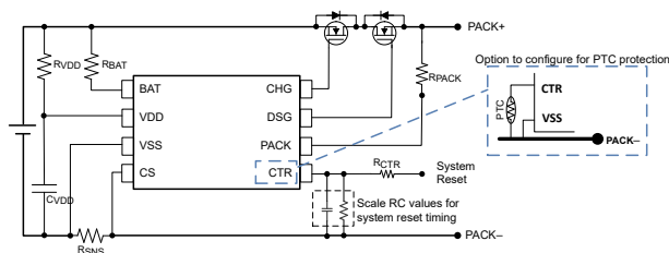
Simplified Schematic
