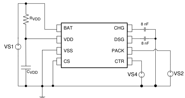
Figure 9-4. Test Circuit 4
