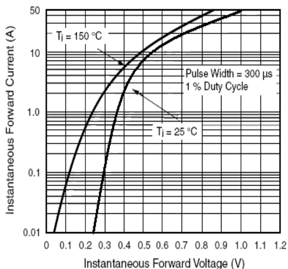
Figure 3. Typical Instantaneous Forward Characteristics Per Diode
