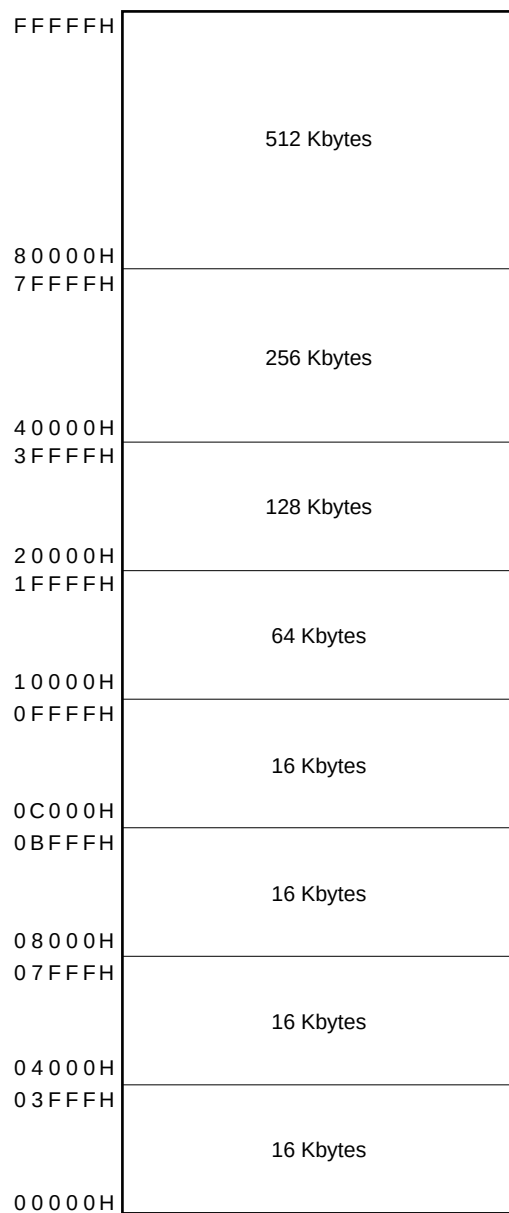
Figure 9-2. Memory Space
