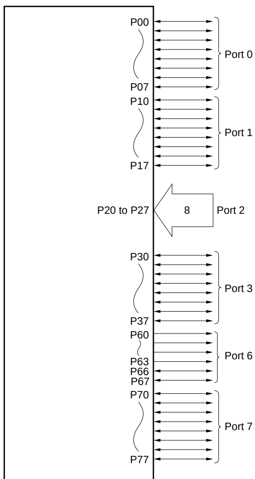
Figure 7-1. Port Configuration
