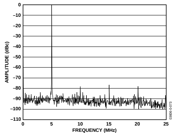
Figure 45. AD9861 Tx Path 5 MHz Single-Tone Output FFT of Tx Path with 2 mA Full-Scale Output into 600 \Omega Differential Load
