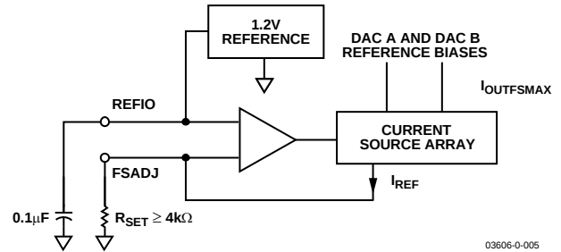
Figure 74. Reference Circuitry
