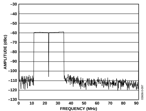
Figure 69. AD9861 Tx Path FFT of OFDM Signal in Figure 52 with 4 \times Interpolation
