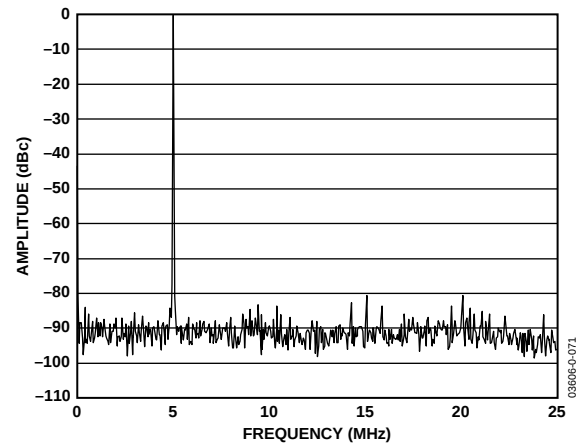
Figure 44. AD9861 Tx Path 5 MHz Single-Tone Output FFT of Tx Path with 20 mA Full-Scale Output into 60 \Omega Differential Load
