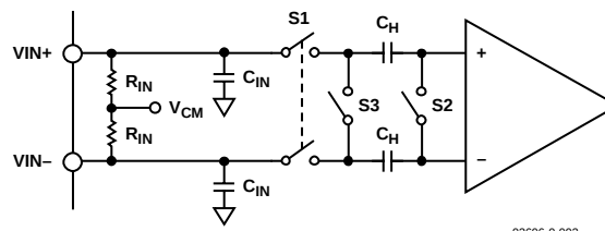
Figure 70. Differential Input Architecture
