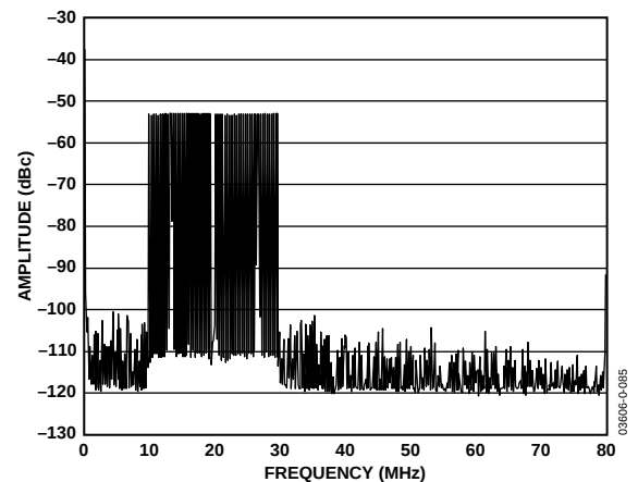
Figure 57. AD9861 Tx Path FFT of OFDM Signal in Figure 52, with 4 \times Interpolation
