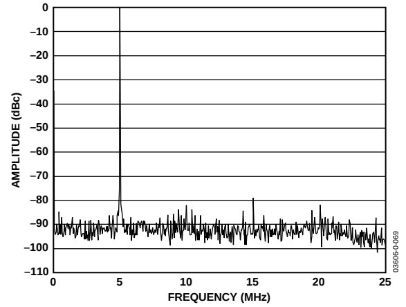
Figure 43. AD9861 Tx Path 5 MHz Single-Tone Output FFT of Tx Path with 20 mA Full-Scale Output into 33 \Omega Differential Load
