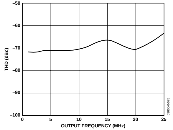
Figure 49. AD9861 Tx Path THD vs. Output Frequency of Tx Path with 2 mA Full-Scale Output into 600 \Omega Differential Load
