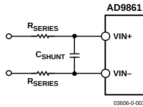
Figure 71. Typical Input
