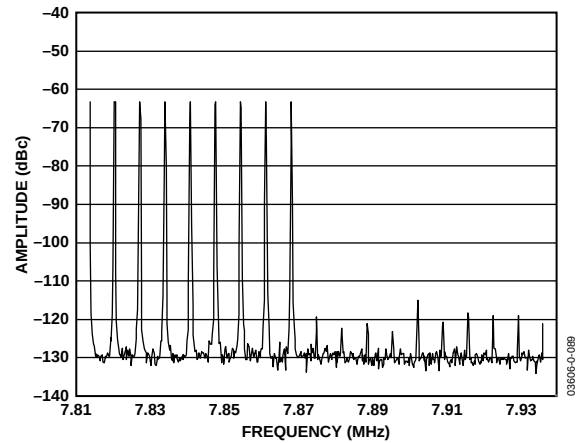
Figure 62. AD9861 Tx Path FFT, Upper-Band IMD Products of OFDM Signal in Figure 52
