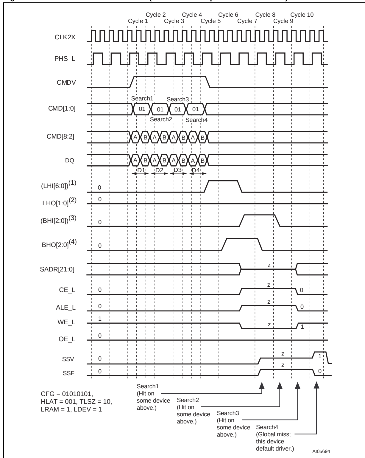
Figure 62. Device 6 in Block Number 3 (Device 30 in Depth-Cascaded Table)
