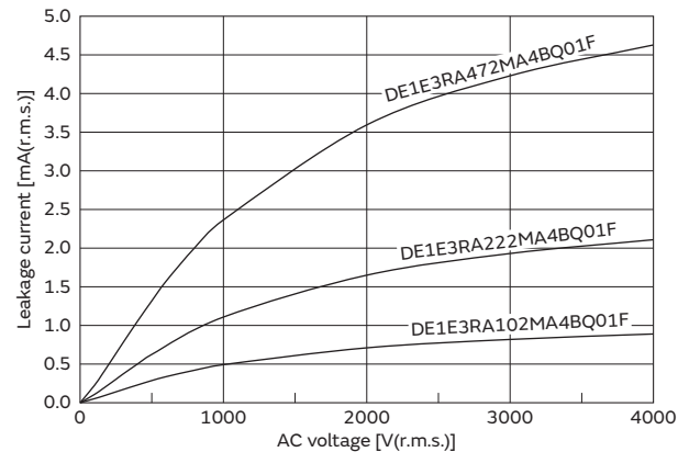
Type RA (AC500V(r.m.s.)) (E char.)
