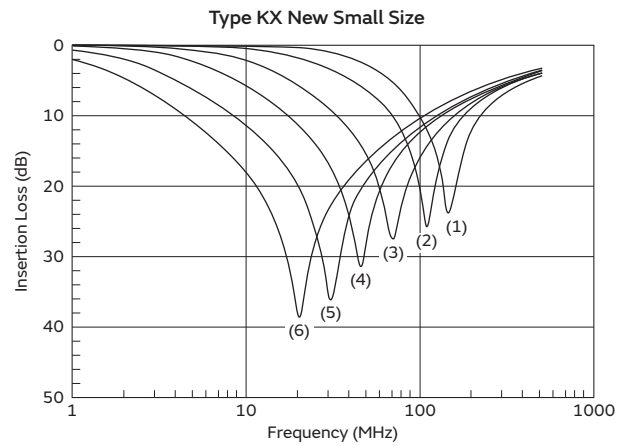
Type KX New Small Size Signal power: 1mW AC240V(r.m.s.) / 60Hz is applied on the capacitor. (1) DE1B3KX101KA4BN01F (2) DE1B3KX221KA4BN01F (3) DE1B3KX471KA4BN01F (4) DE1E3KX102MA4BN01F (5) DE1E3KX222MA4BN01F (6) DE1E3KX472MA4BN01F
