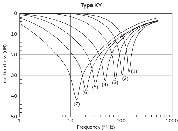
Type KY Signal power: 1mW AC240V(r.m.s.) / 60Hz is applied on the capacitor. (1) DE2B3KY101KA2B**** (2) DE2B3KY221KA2B**** (3) DE2B3KY471KA2B**** (4) DE2E3KY102MA2B**** (5) DE2E3KY222MA2B**** (6) DE2E3KY472MA2B**** (7) DE2F3KY103MA3B****
