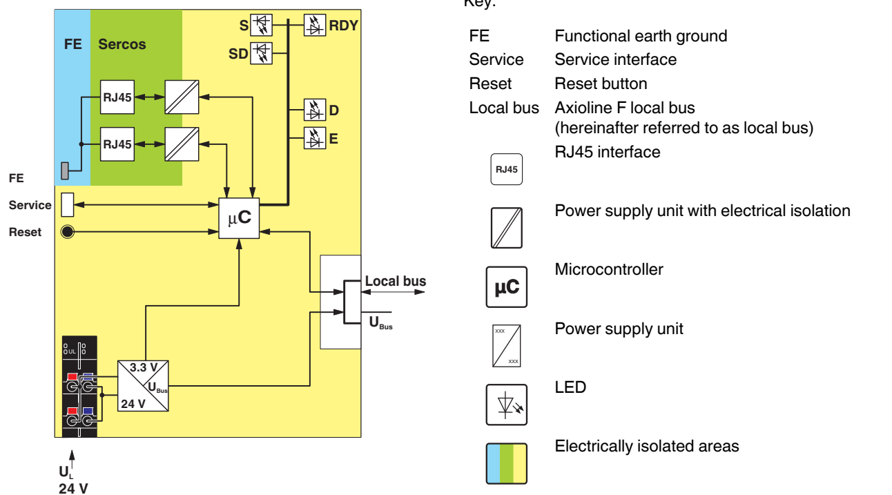
Figure 1 Internal wiring of the terminal points
