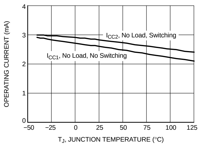
Figure 30. Operating Supply Current vs. Temperature
