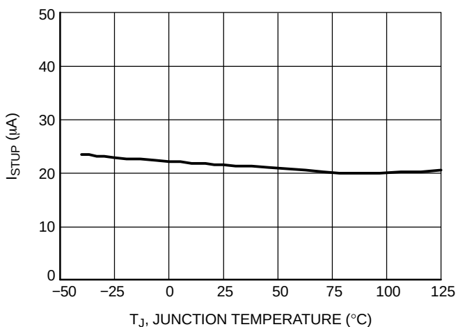
Figure 28. Supply Current in Startup Mode vs. Temperature
