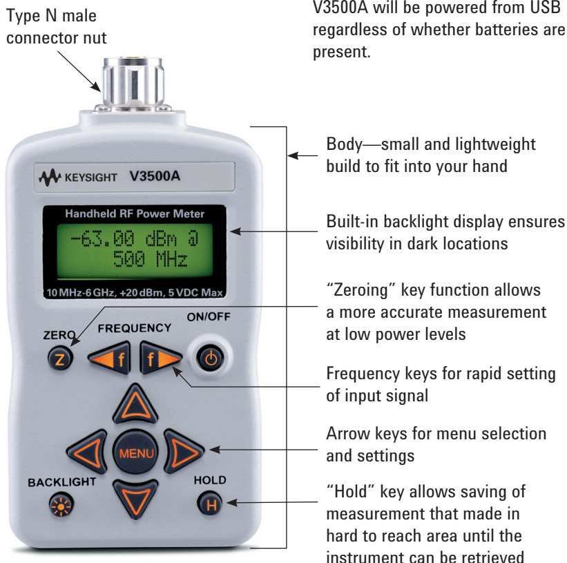
Figure 1. Signal connection
