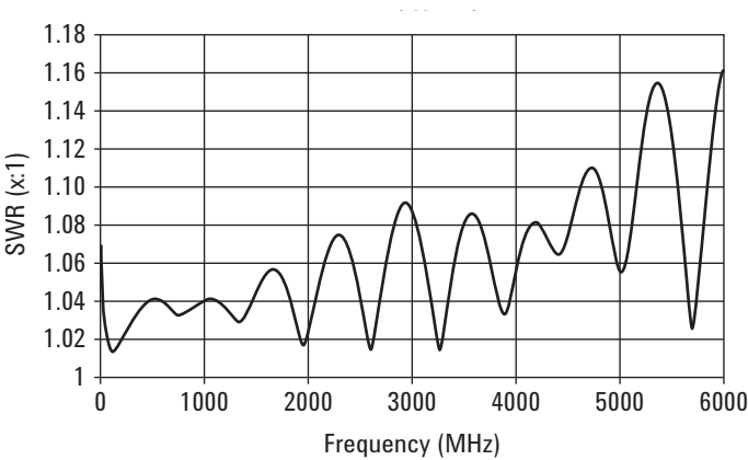
Typical SWR performance
