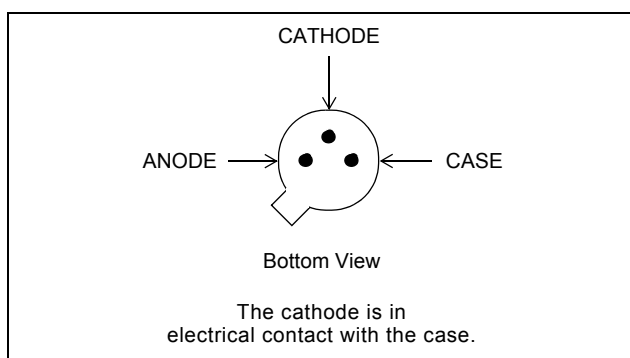
Figure 1 - Pin Diagram
