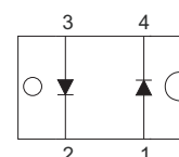
Anti-Parallel NST120F06-A
