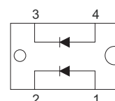
Parallel NST120F06
