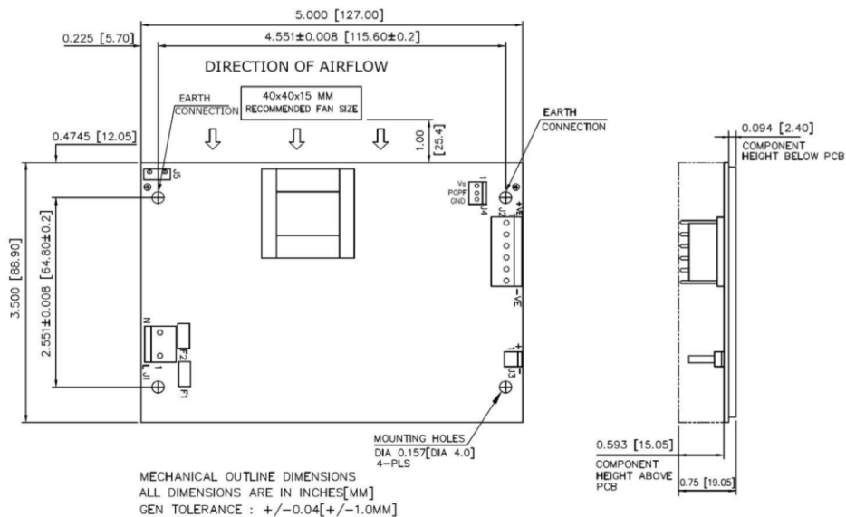
Mechanical Drawing – Option 2 with PGPF
