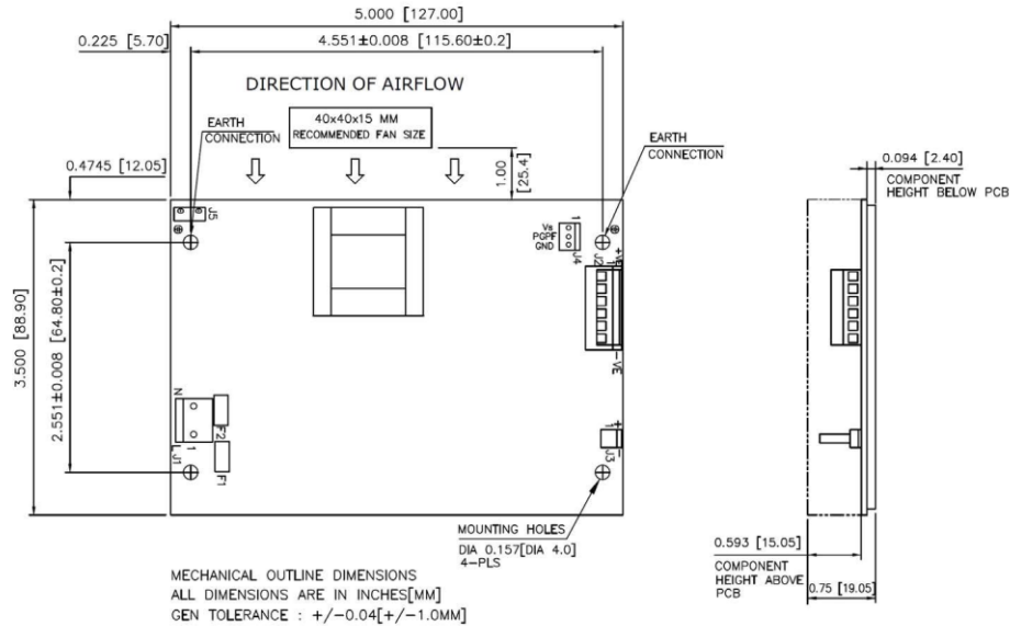
Mechanical Drawing – Option 1 with PGPF
