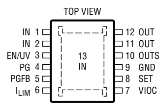
MSE PACKAGE 12-LEAD PLASTIC MSOP T_{JMAX} = 150^{\circ}\text{C} , \theta_{JA} = 33^{\circ}\text{C/W} , \theta_{JC} = 8^{\circ}\text{C/W} EXPOSED PAD (PIN 13) IS IN, MUST BE SOLDERED TO PCB
