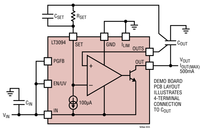
Figure 3. C OUT and C SET Connections for Best Performance
