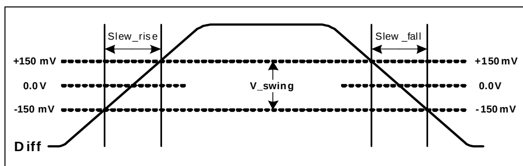
Figure 2-5. Differential Measurements
