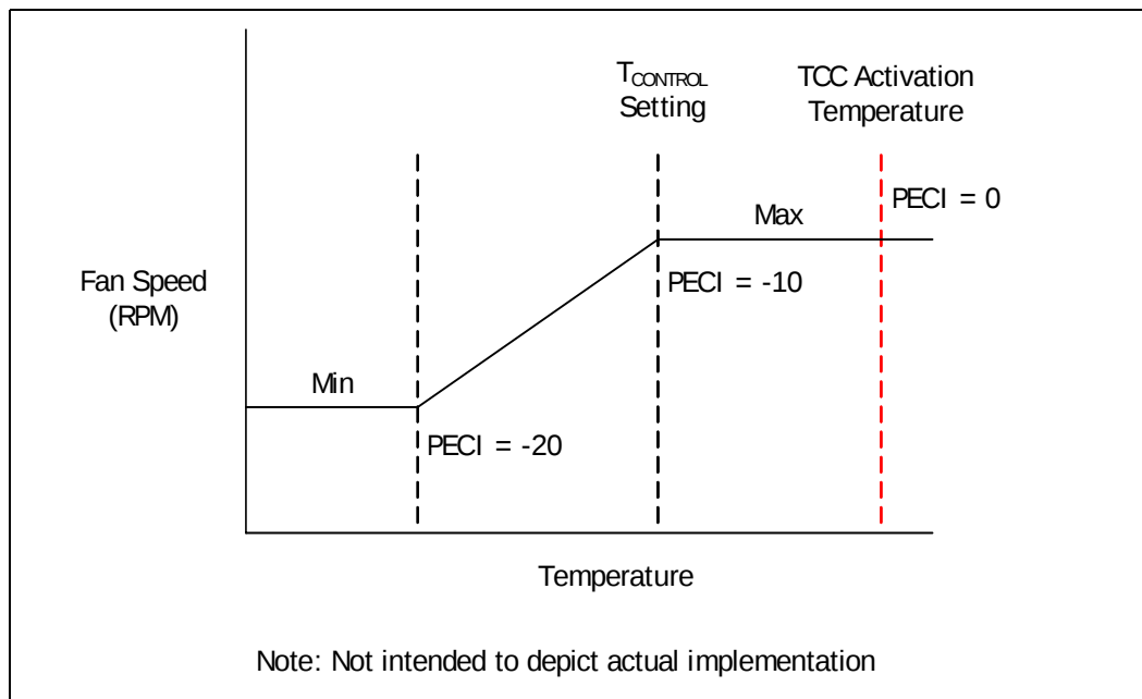
Figure 5-4. Conceptual Fan Control on PECI-Based Platforms
