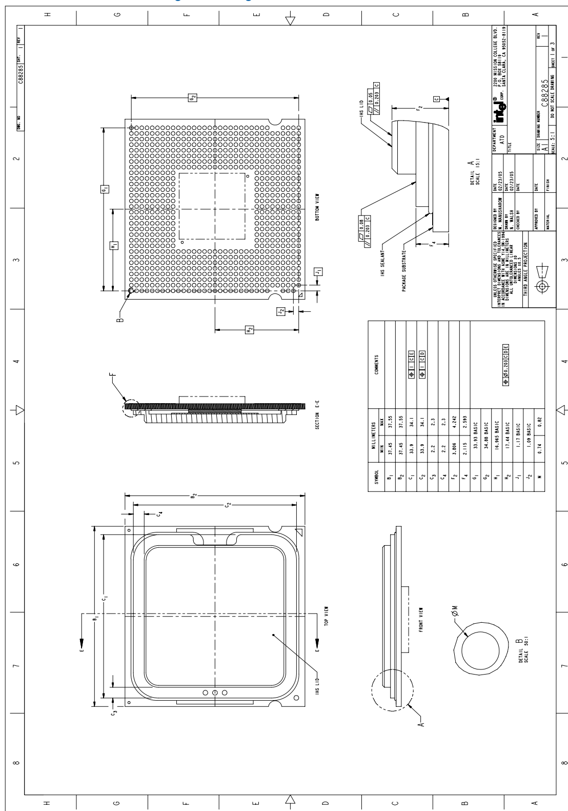
Figure 3-2. Processor Package Drawing Sheet 1 of 3
