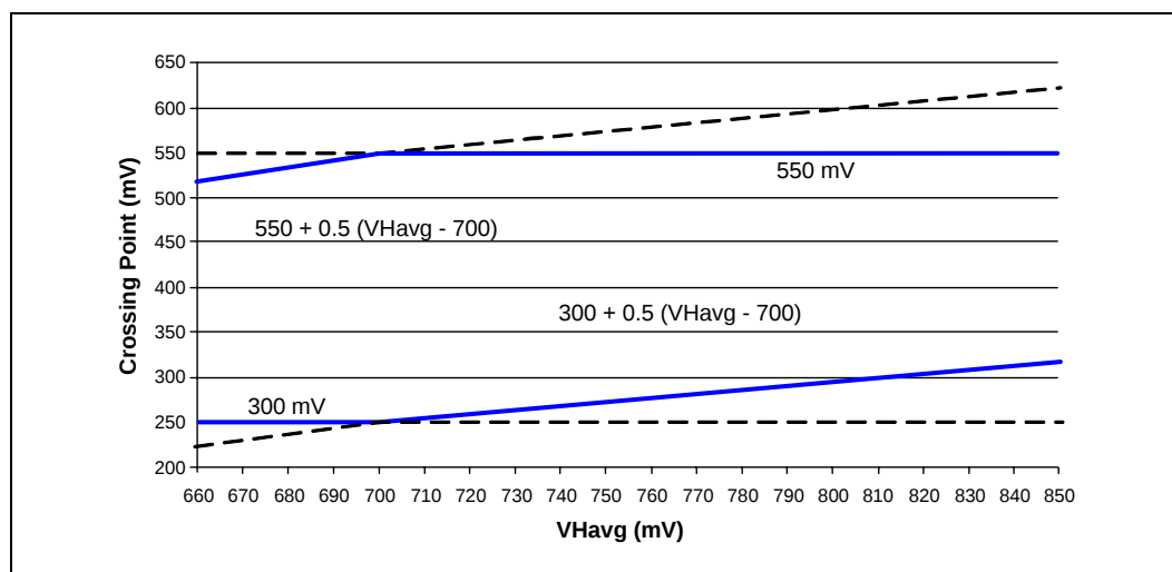
Figure 2-5. Differential Measurements
