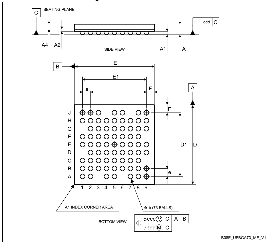
Figure 33. UFBGA73 - Outline
