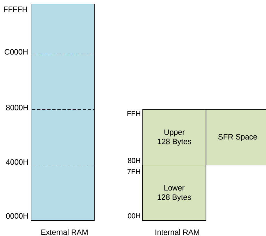
Figure 5. Memory Space
