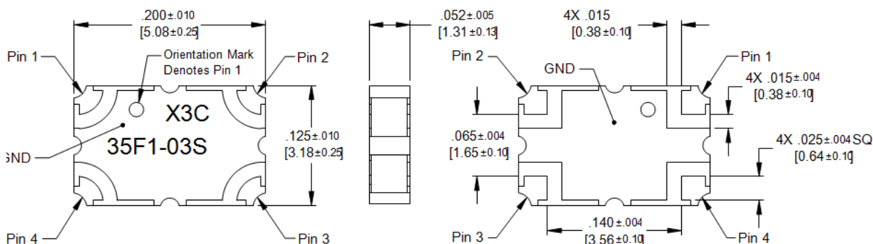
Dimensions are in Inches [Millimeters] X3C35F1-03S Mechanical Outline
