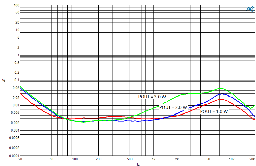
Figure 6: THD versus frequency ( 4\ \Omega + 33\ \mu\text{H} ) 4.5 V
