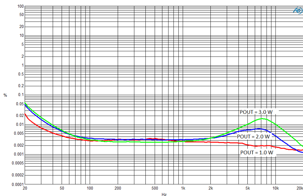
Figure 9: THD versus frequency (8 \Omega + 33 \mu H) 9.0 V
