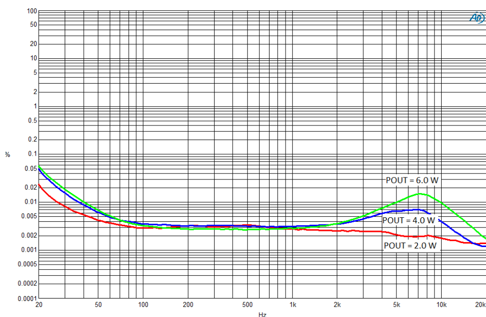
Figure 10: THD versus frequency (4 \Omega + 33 \mu H) 9.0 V
