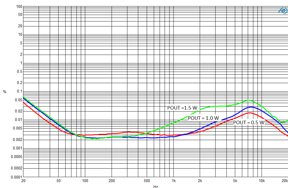
Figure 5: THD versus frequency ( 8\ \Omega + 33\ \mu\text{H} ) 4.5 V
