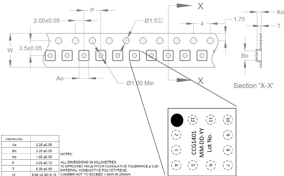
Figure 9: CSP Tape Dimensions
