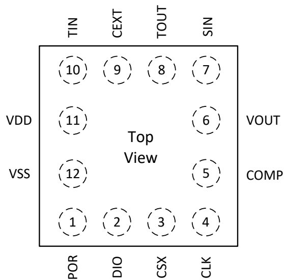
Figure 3: CCG1401 Pad configuration (CSP/Bumped Die)
