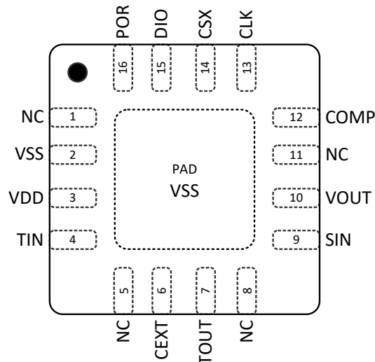
Figure 2: CCG1401 - QFN16 (Top View)
