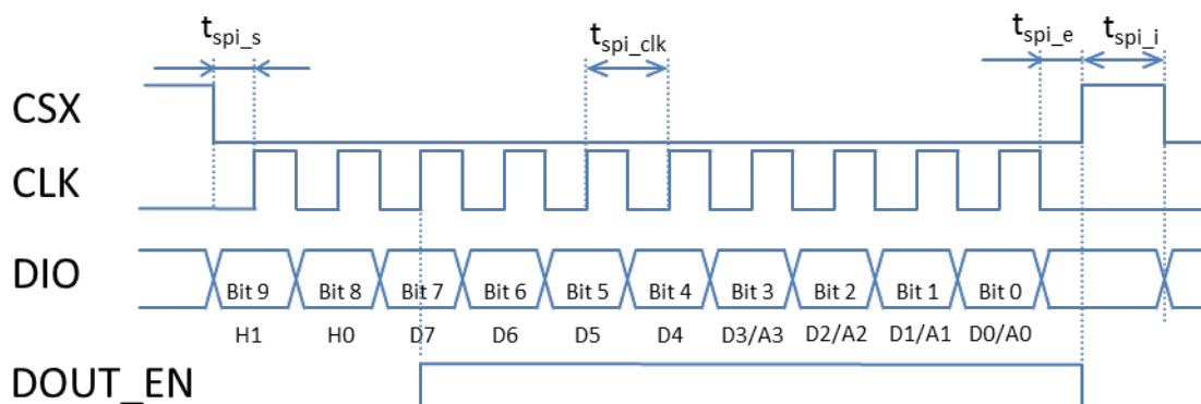
Figure 4: Timing diagram
