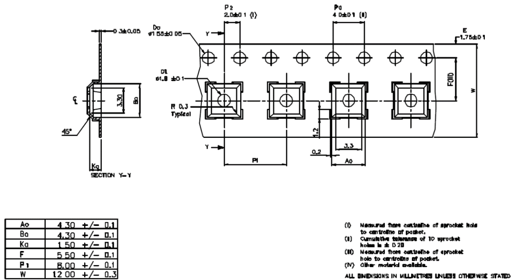
Figure 8: QFN16 Tape Dimensions
