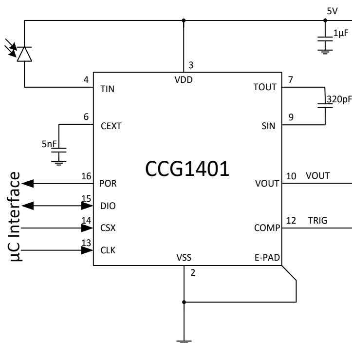
Figure 4: Optical Application
