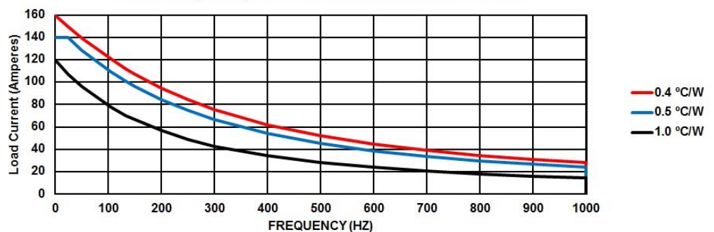
PWM frequency vs. Load Current HDC200D160
