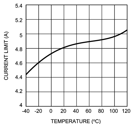
Current Limit vs Temp
