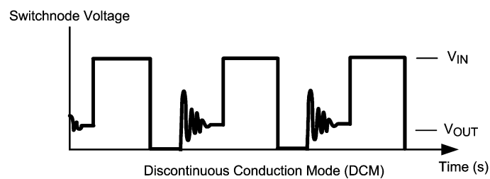
FIGURE 6. Modes of Operation
