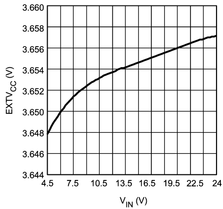
EXTV CC vs V IN
