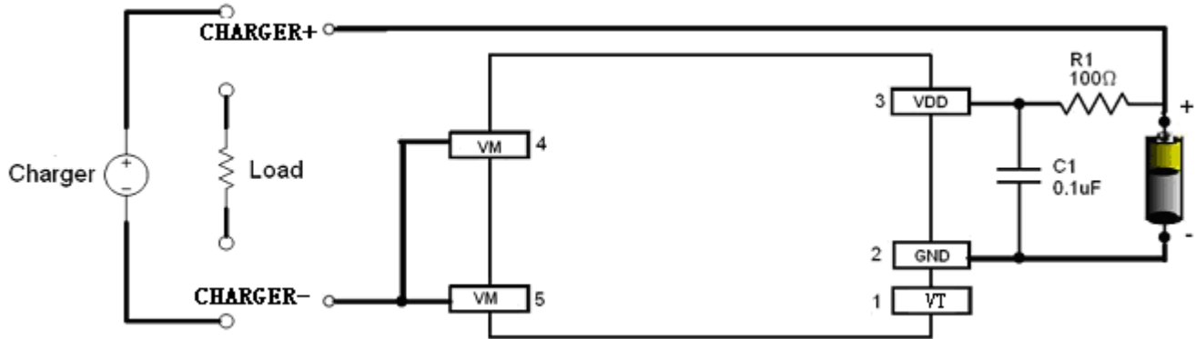
Fig 6 HM5456 in a Typical Battery Protection Circuit
