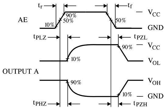
Figure 3. Switching Waveforms
