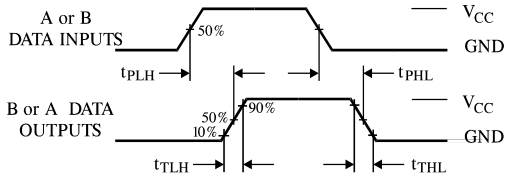
Figure 1. Asynchronous operation
