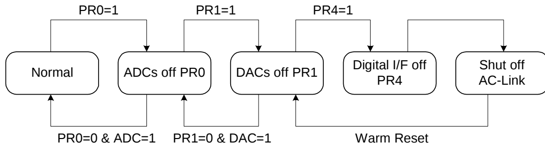
Figure 20. STAC9750/9751 Powerdown/Powerup Flow With Analog Still Active
