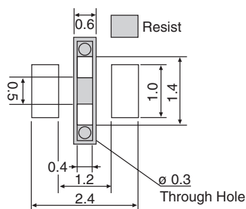
0603 Chip Mounting Side
