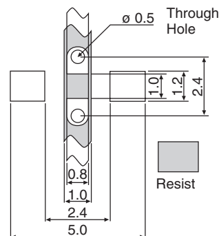
1206 Chip Mounting Side
