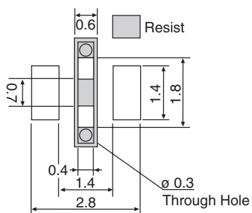
0805 Chip Mounting Side
