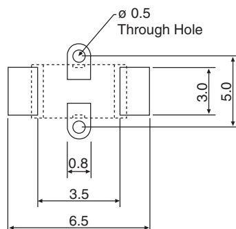
1812 Chip Mounting Side
