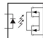
1-Form-A Bidirectional
