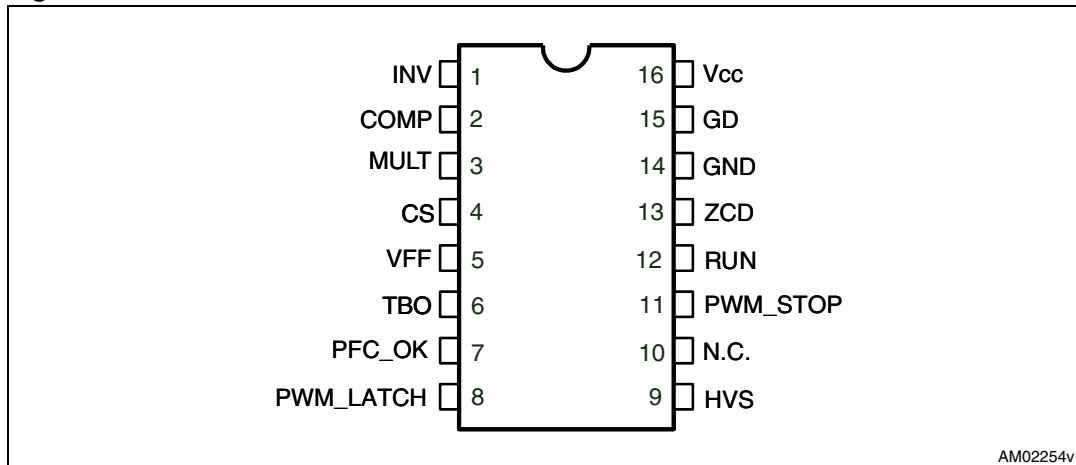
Figure 2. Pin connection
