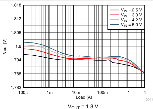
图 9-12. Load Regulation
