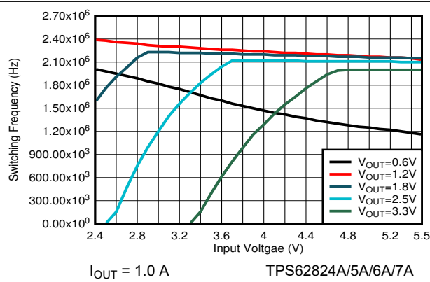
图 9-26. Switching Frequency
