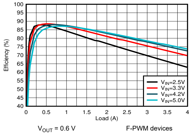
图 9-5. PWM Efficiency
