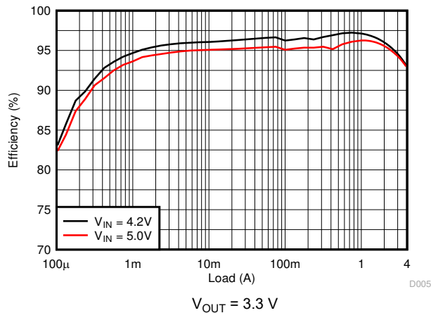
图 9-19. Efficiency
