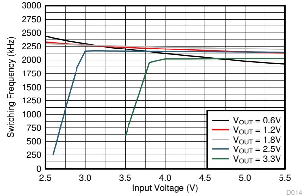
图 9-28. Switching Frequency
