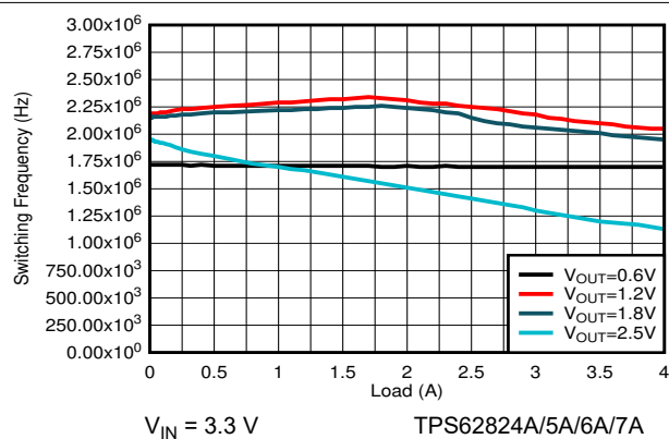
图 9-25. Switching Frequency
