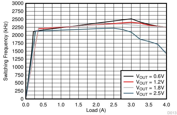
图 9-27. Switching Frequency
