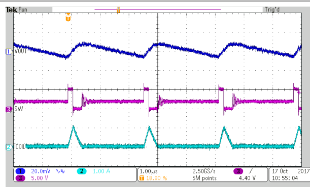
图 9-34. PSM Operation
