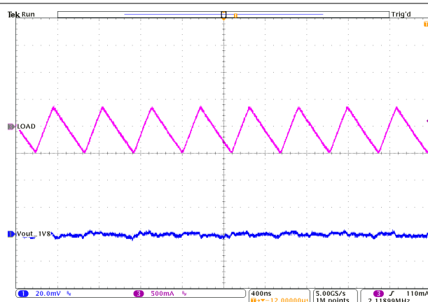
图 9-34. PSM Operation
