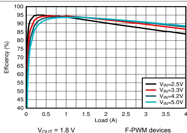
图 9-13. PWM Efficiency
