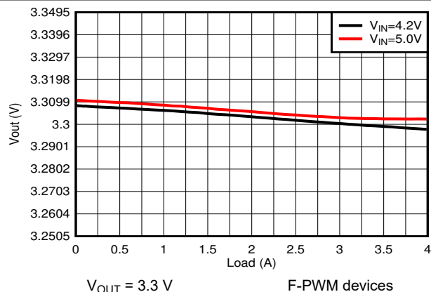
图 9-22. Load Regulation
