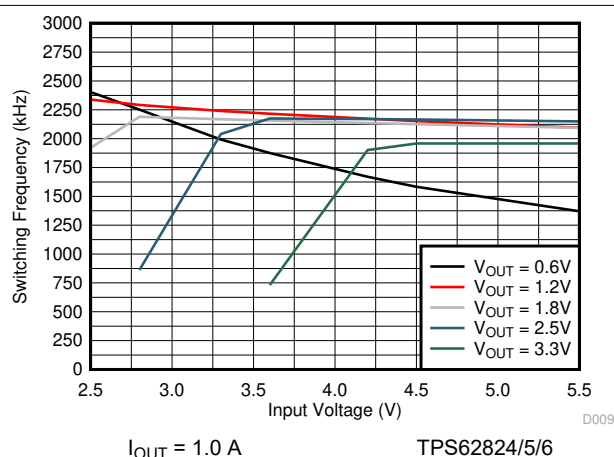
图 9-24. Switching Frequency
