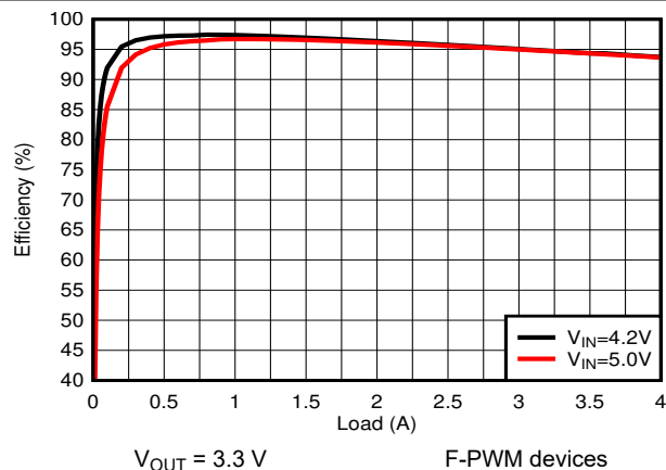
图 9-21. PWM Efficiency
