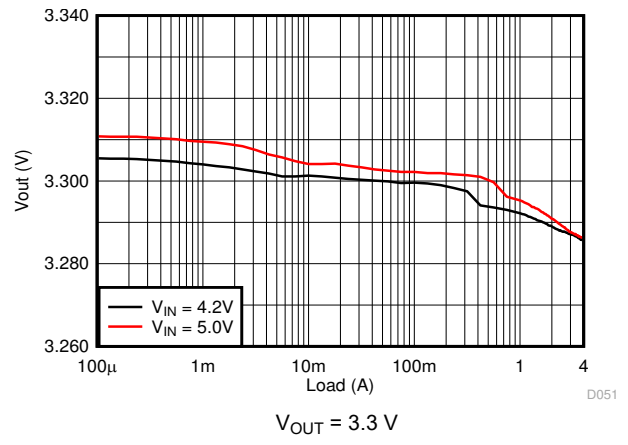
图 9-20. Load Regulation
