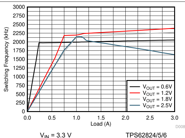
图 9-23. Switching Frequency
