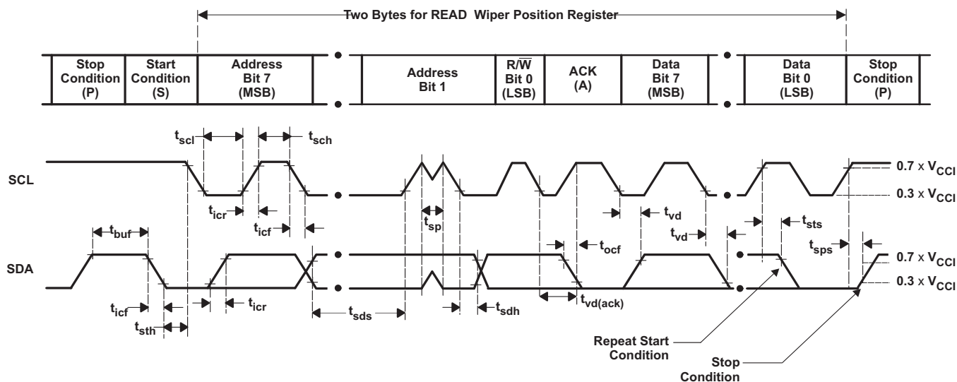
VOLTAGE WAVEFORMS
