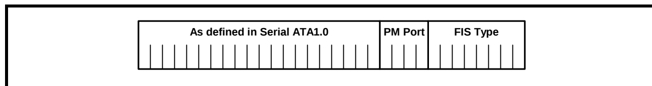
FIGURE 9. PORT SELECTION SIGNAL - TRANSMITTED COMRESET SIGNALS
