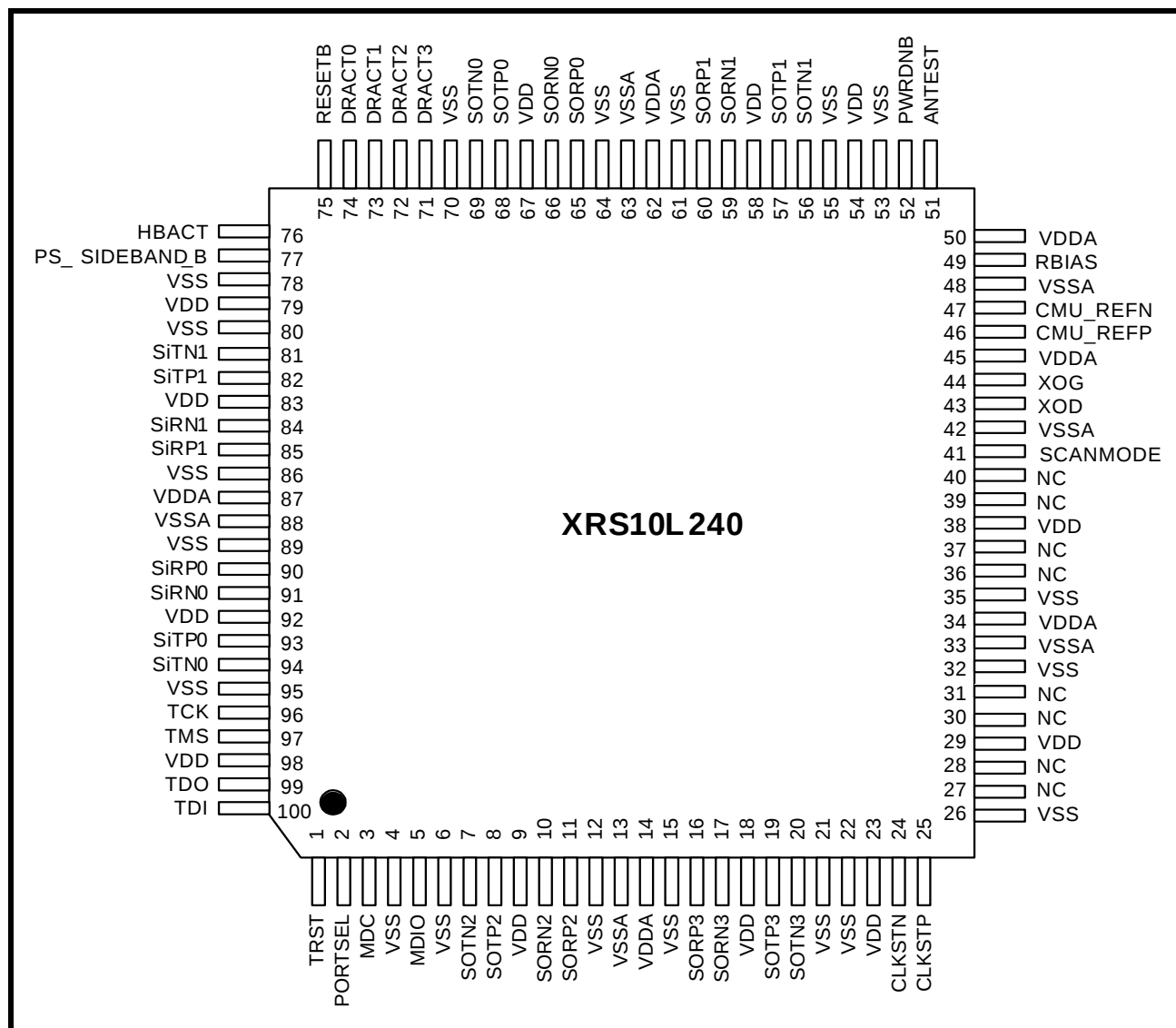
FIGURE 2. PINOUT OF THE XRS10L240
