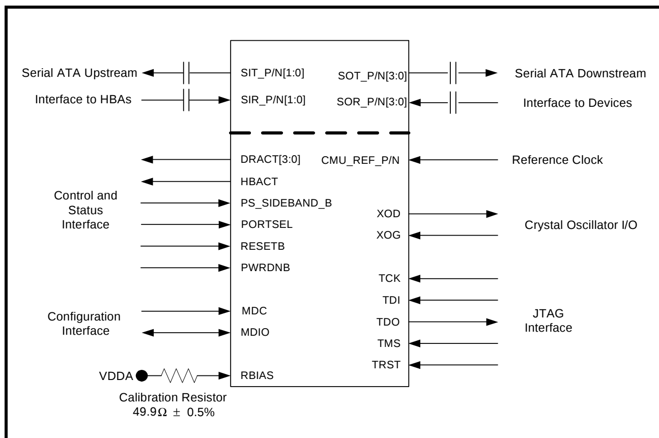
FIGURE 3. XRS10L240 INTERFACES
