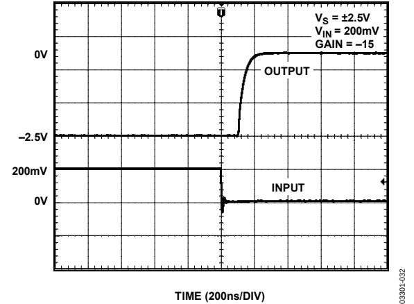
Figure 32. Positive Overload Recovery Time
