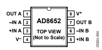
Figure 4. 8-Lead SOIC_N (R-8)
