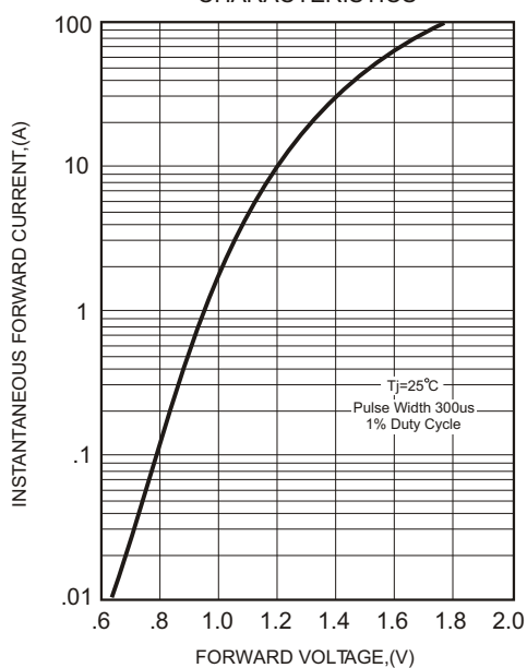
FIG.1-TYPICAL FORWARD
