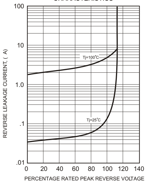
FIG.3 - TYPICAL REVERSE
