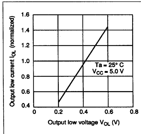
Output Current vs. Output Voltage (Low)
