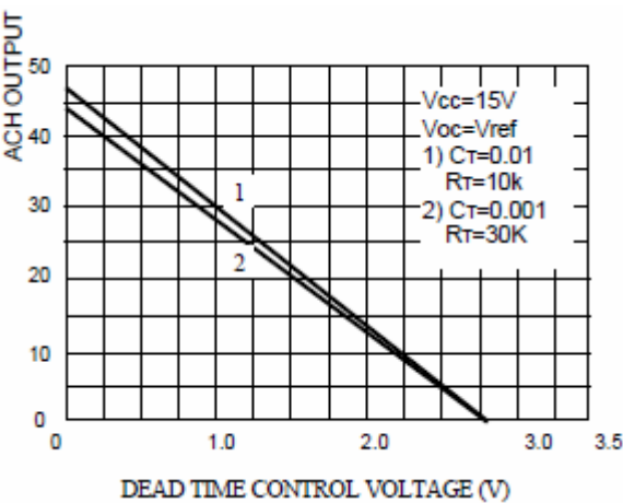
FIGURE 4 – PERCENT DUTY CYCLE vs. DEAD-TIME CONTROL VOLTAGE
