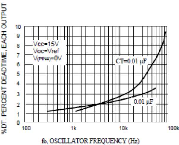
FIGURE 3 – PERCENT DEAD TIME vs. OSCILLATOR FREQUENCY
