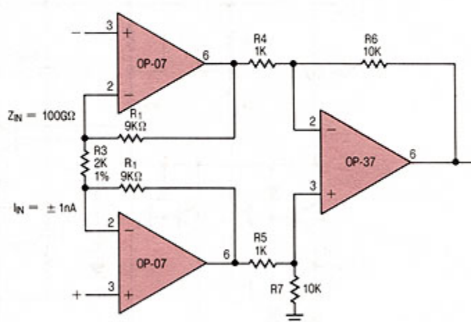
Instrumentation Amplifier
