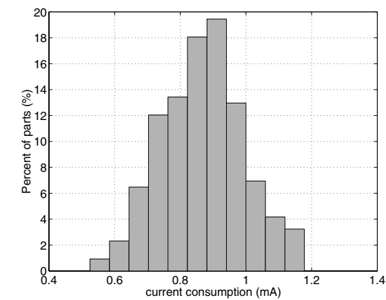
Figure 19. Current consumption at 3.3V
