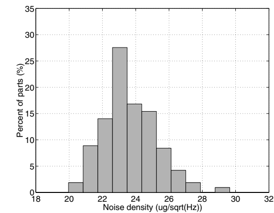
Figure 17. Noise density at 3.3V (x,y axes)
