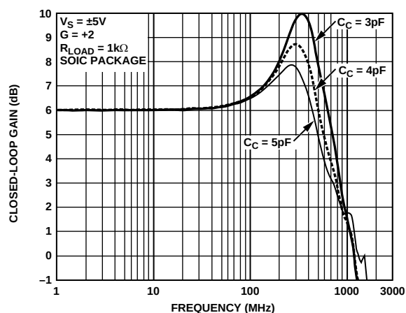
Figure 73. Frequency Response for Various Values of C_C
