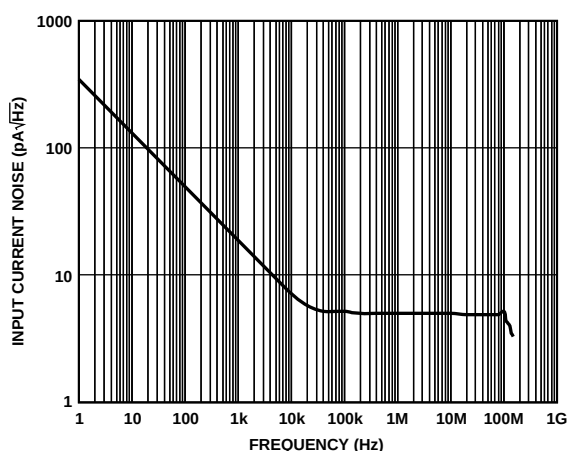
Figure 51. Input Current Noise vs. Frequency ( \overline{DISABLE} = +V_S )
