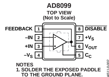
Figure 2. 8-Lead SOIC-EP (RD-8-1)
