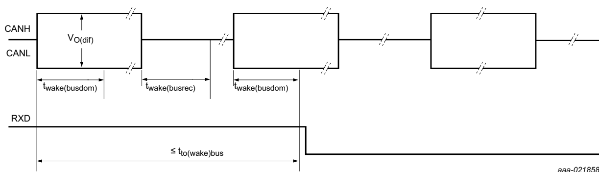
Fig 5. Wake-up timing
