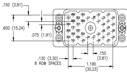
38 PIN PLUG
