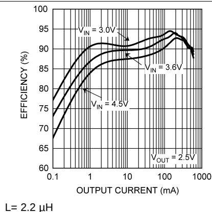
Figure 13. Efficiency vs. Output Current
