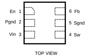
6 Pins USON Package (NKH) TOP VIEW
