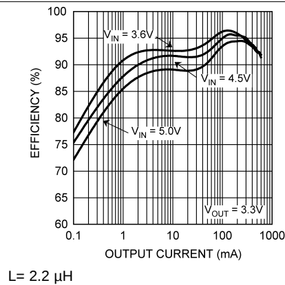
Figure 14. Efficiency vs. Output Current
