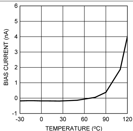
Figure 3. Feedback Bias Current vs. Temp
