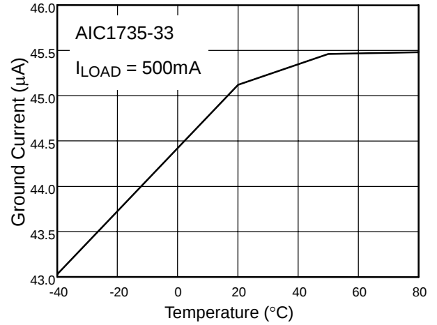
Fig. 8 Ground Current vs. Temperature
