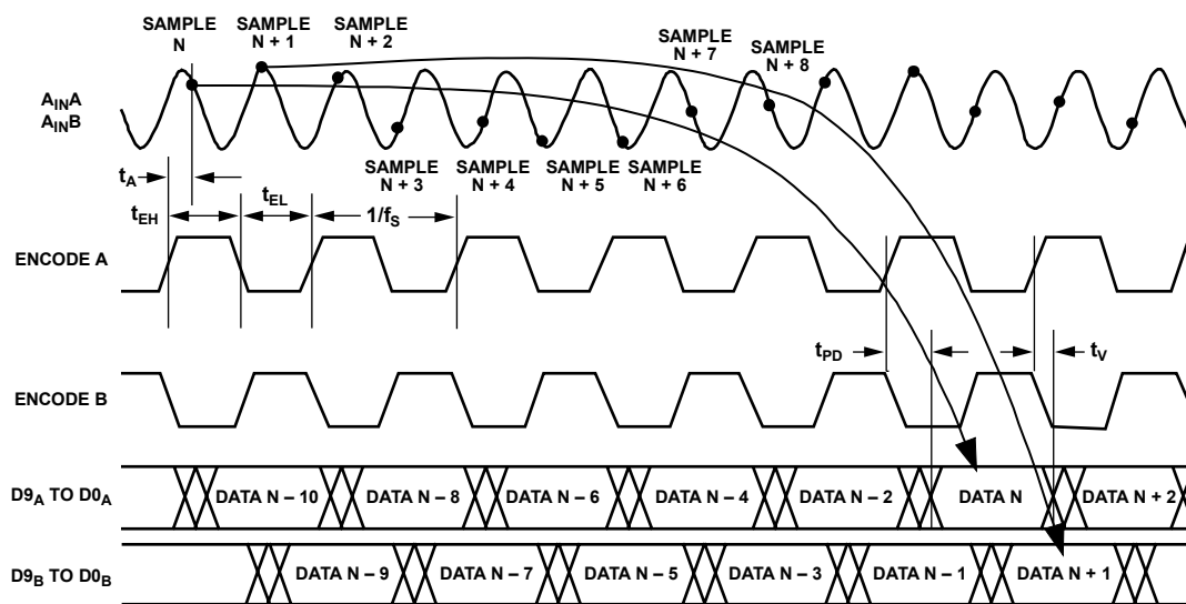
Figure 3. Normal Operation with Two Clock Sources ( S1 = 1, S2 = 0 ) Channel Timing
