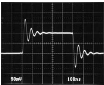
Small-Signal Transient (Noninverting, G = 1 , C_L = 100pF )
