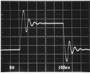
Large-Signal Transient (Noninverting, G = 1 , C_L = 100pF )
