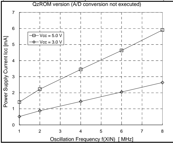
Fig. 14. f(XIN) -Icc (Double-speed mode)
