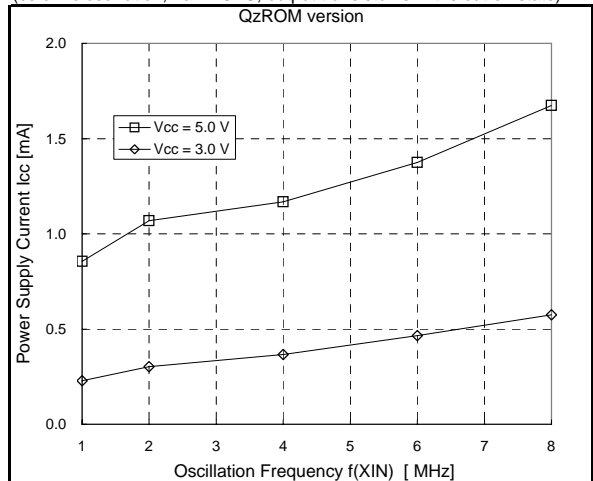
Fig. 17. f(XIN) -Icc (At WIT instruction executed)
