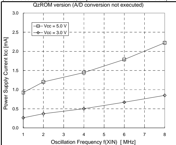
Fig. 16. f(XIN) -Icc (Middle-speed mode)
