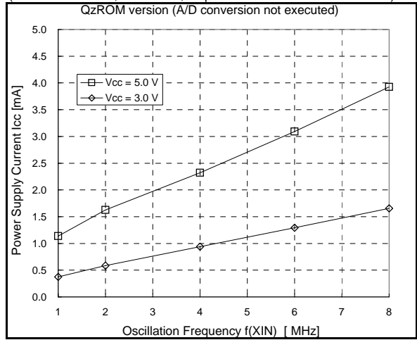
Fig. 15. f(XIN) -Icc (High-speed mode)
