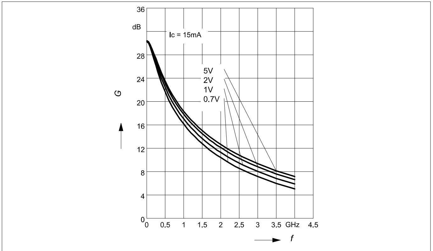
Figure 6 Transducer Gain IS_{21}^2 = f(f), I_C = 15 mA, V_{CE} = parameter
