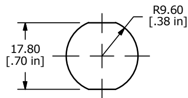
PANEL CUT-OUT PANEL THICKNESS 1-10mm
