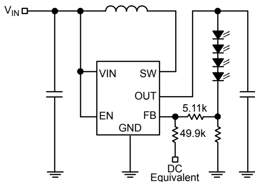
Figure 2. Continuous Dimming
