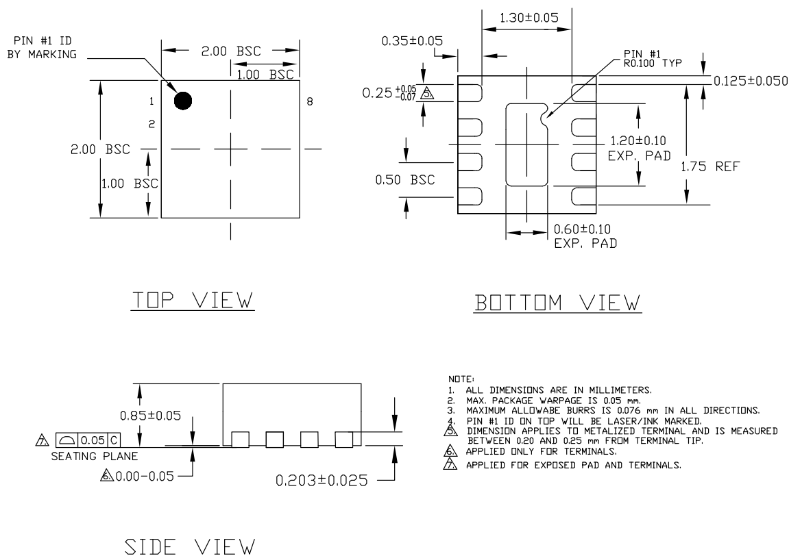
8-Pin MLF ® (ML)
