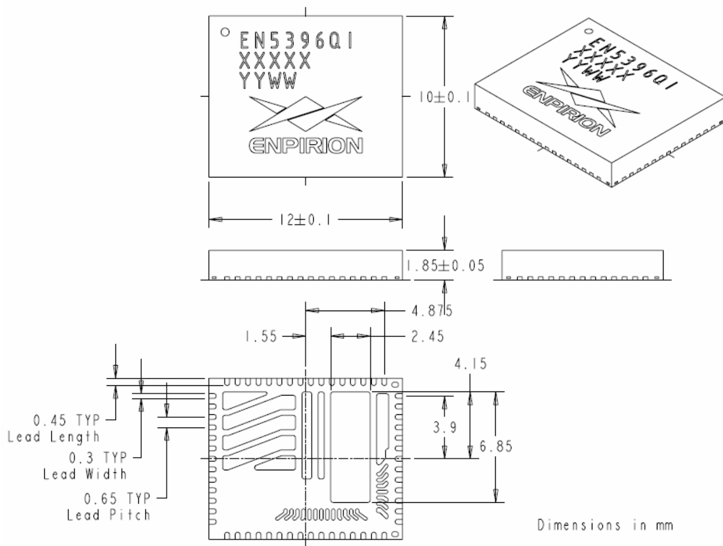
Figure 11. Package dimensions.
