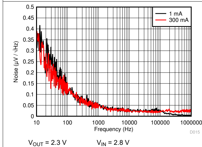
Figure 6-15. Noise Density
